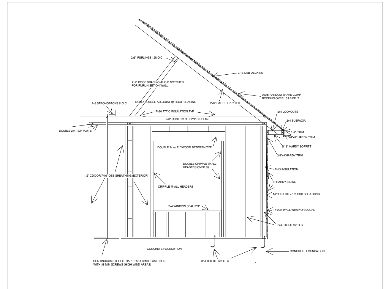
TYPICAL WALL DETAIL
