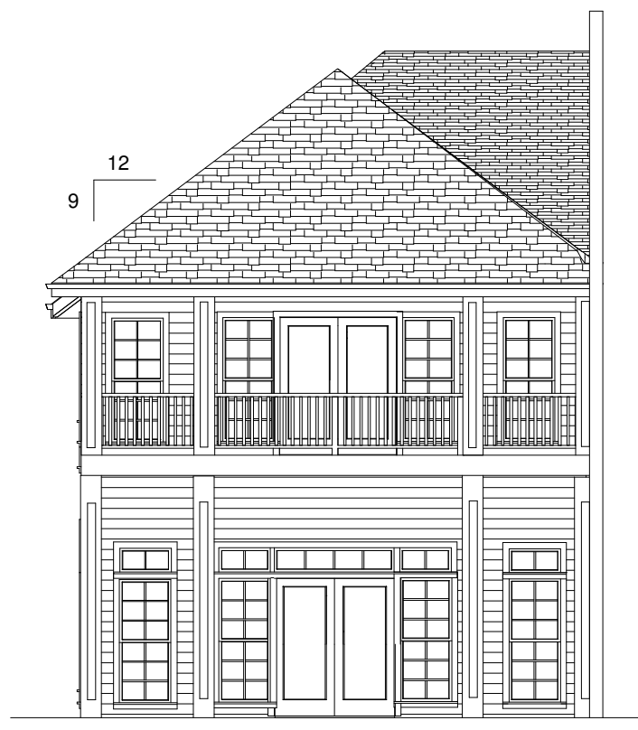
REAR ELEVATION
